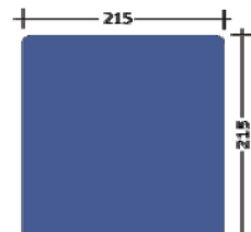
SQU-215-215-R10-00
